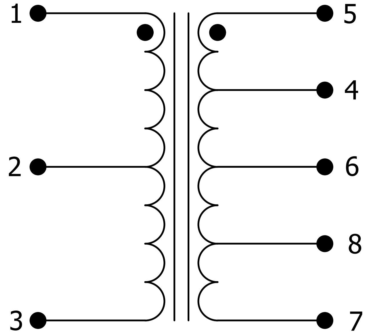
CIRCUIT DIAGRAM FOR 68515 ONLY
