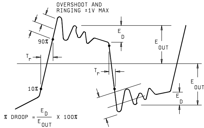
FIGURE 4. Output wave form for test circuit on figure 3.
