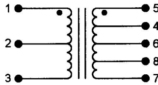
CIRCUIT DIAGRAM FOR DASH NUMBER -19
